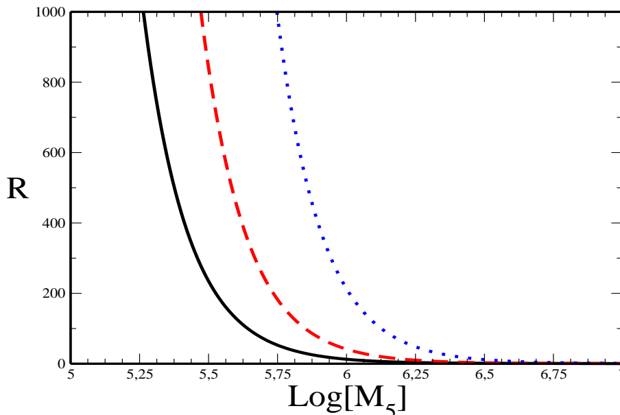
Figure 1: The enhancement/suppression factor R = (\Omega_\chi h^2)_b / (\Omega_\chi h^2)_s as a function of the five dimensional scale M_5 (GeV) for m_\chi = 100 (solid curve), 200 (dashed curve) and 500 GeV (dotted curve).
